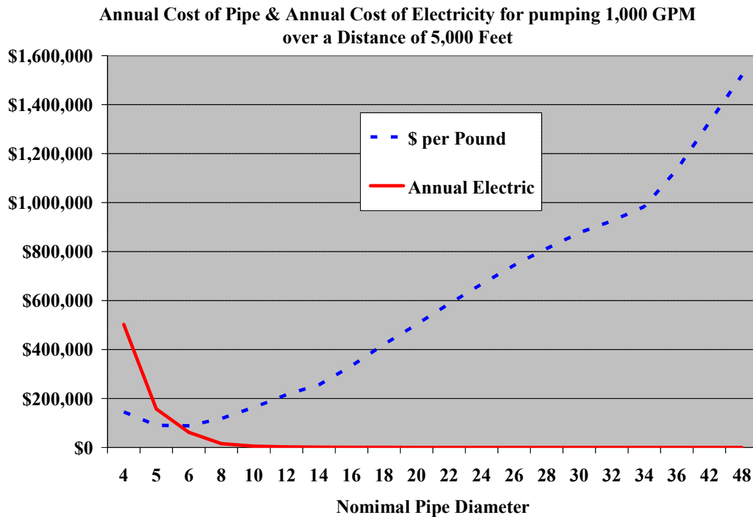
Graph 6. Annual Loan Payment for Pipe and Annual Electric Cost
