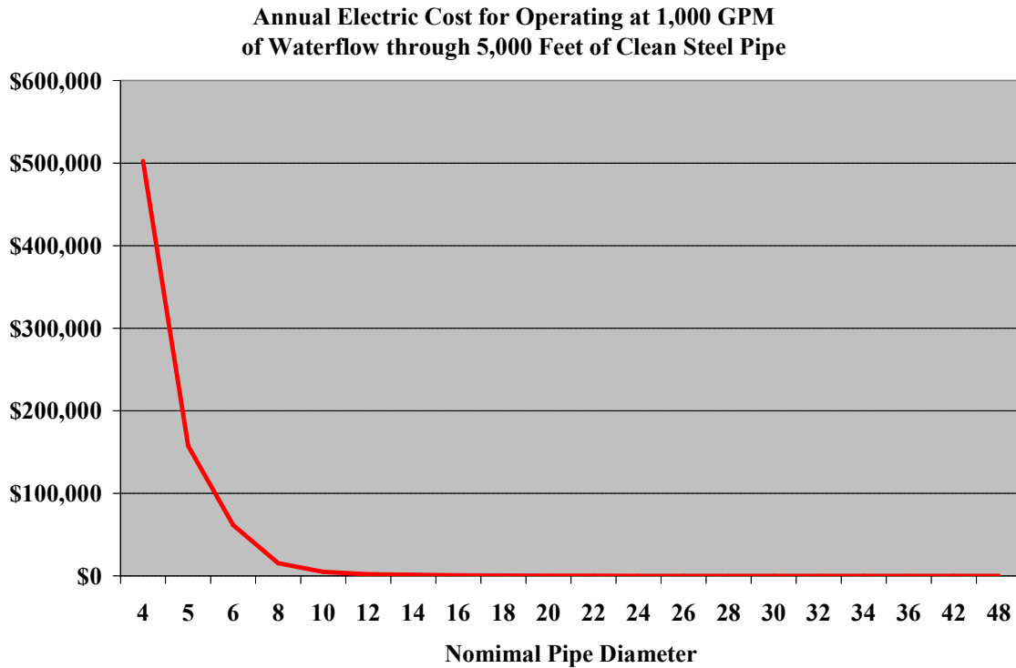
Graph 4. Annual Electricity Cost for Operating the Pump Motor
