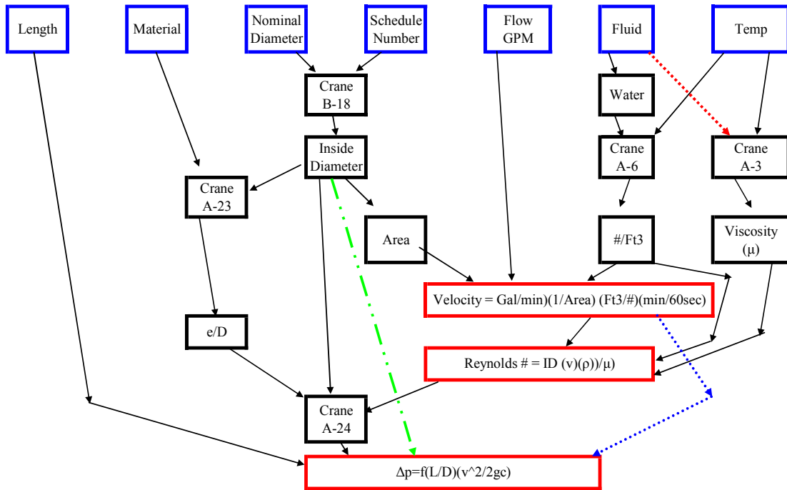
Figure 1. Flow Charting the Pressure Drop Equations
