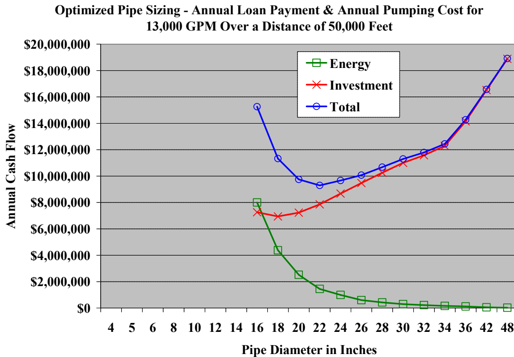
Graph 16. Optimized Pipe Diameter for 13,000 GPM and 50,000 Feet Distance
