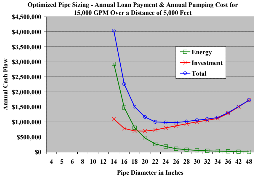
Graph 10. Optimized Pipe Pump Sizing for 15,000 GPM
