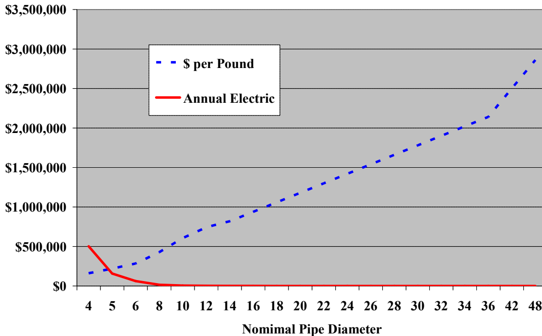
Graph 5. Capital Cost of Pipe and Annual Electric Cost as a Function of Pipe Diameter
