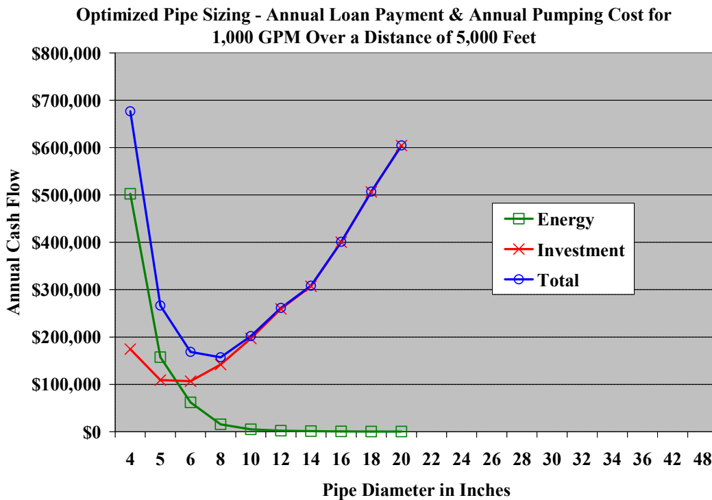
Graph 7. Optimized Pipe Pump Sizing for 1,000 GPM
