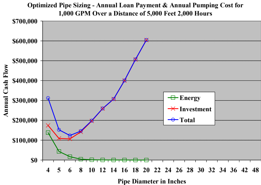
Graph 14. Optimized Pipe Pump Sizing for 1,000 GPM Operating 2,000 Hours
