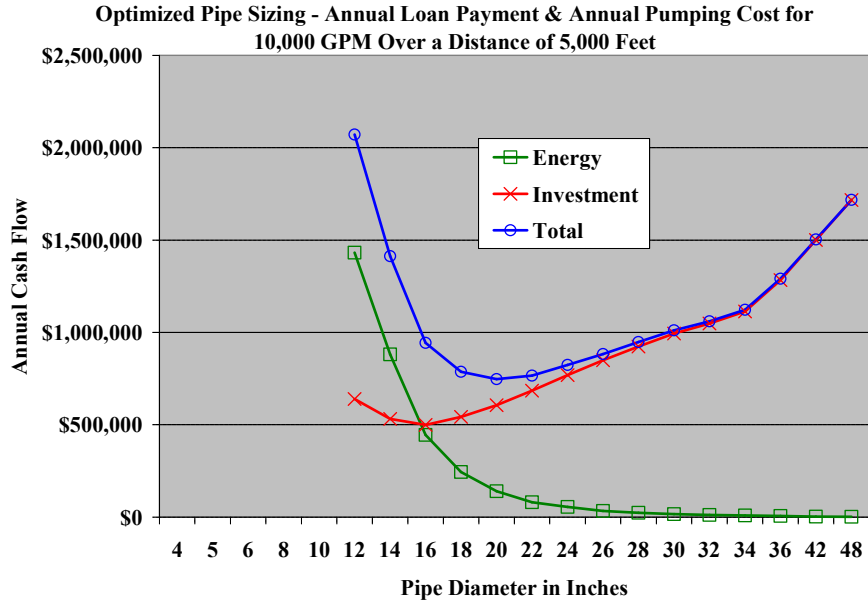
Graph 9. Optimized Pipe Pump Sizing for 10,000 GPM
