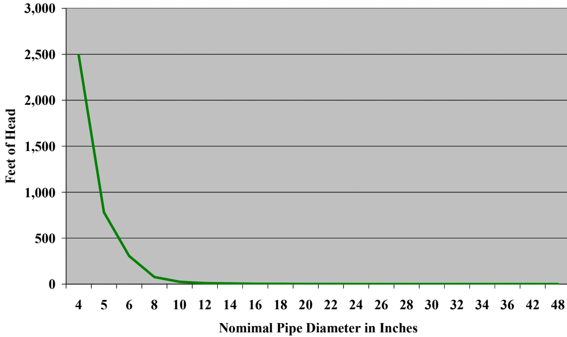
Graph 2. Head Loss as a Function of Pipe Diameter
