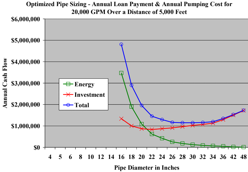
Graph 11. Optimized Pipe Pump Sizing for 20,000 GPM
