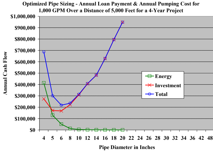
Graph 12. Optimized Pipe Pump Sizing for 1,000 GPM and 4-year Project Life
