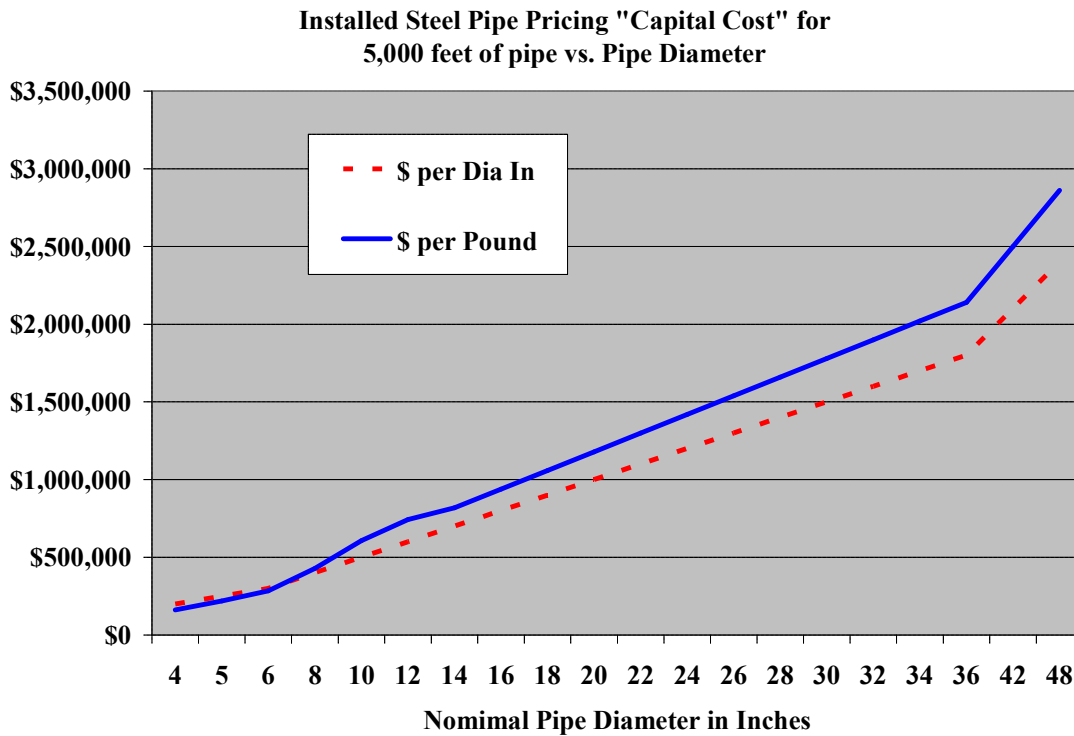
Graph 3. Installed Pipe Cost as a Function of Diameter
