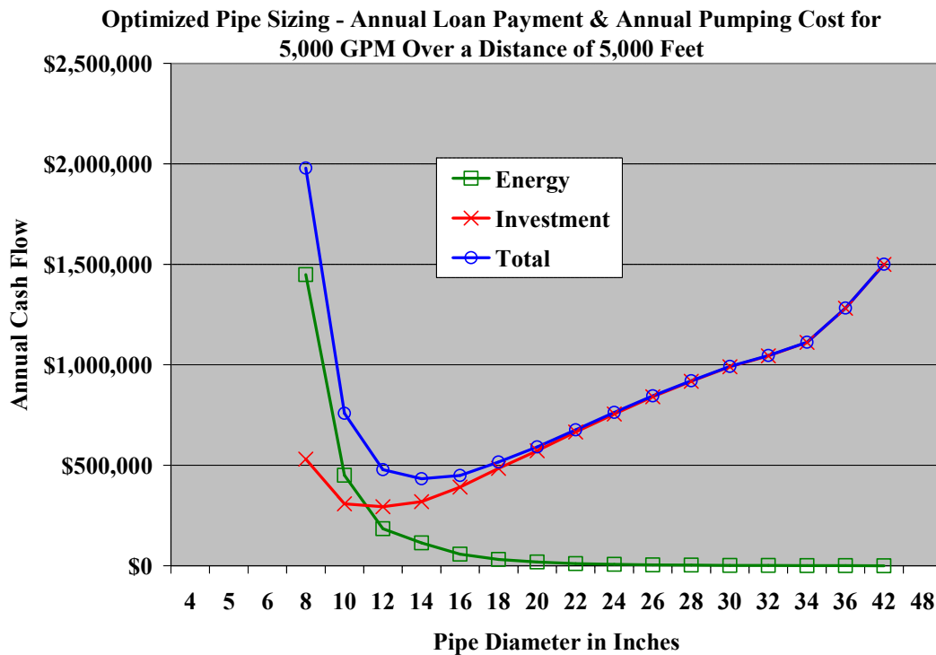
Graph 8. Optimized Pipe Pump Sizing for 5,000 GPM
