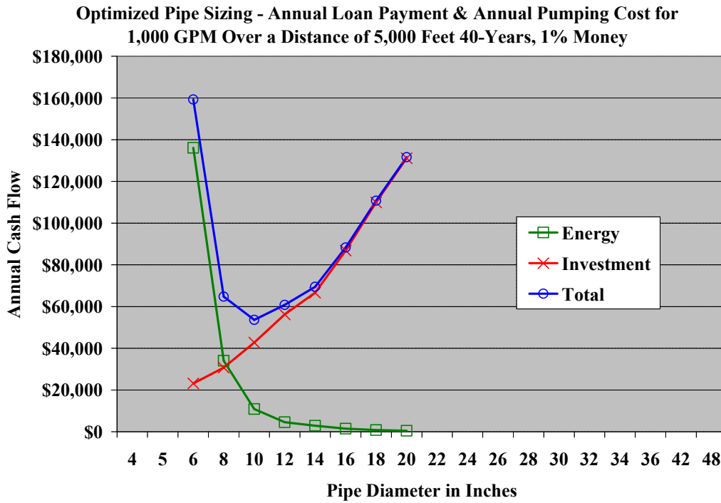
Graph 15. Optimized Pipe Pump Sizing for 1,000 GPM 40-Years, 1% Money
