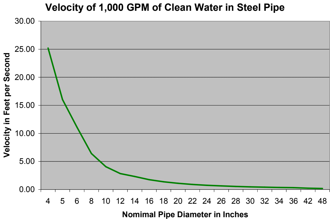
Graph 1. Fluid Velocity as a Function of Pipe Diameter
