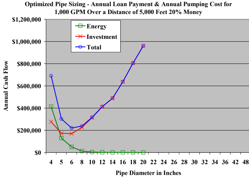
Graph 13. Optimized Pipe Pump Sizing for 1,000 GPM and an Interest Rate of 20%
